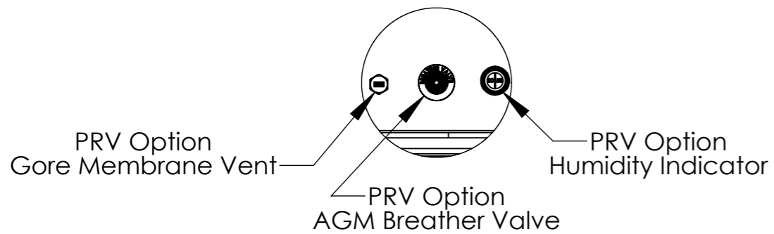
DETAIL A SCALE 1 : 5
